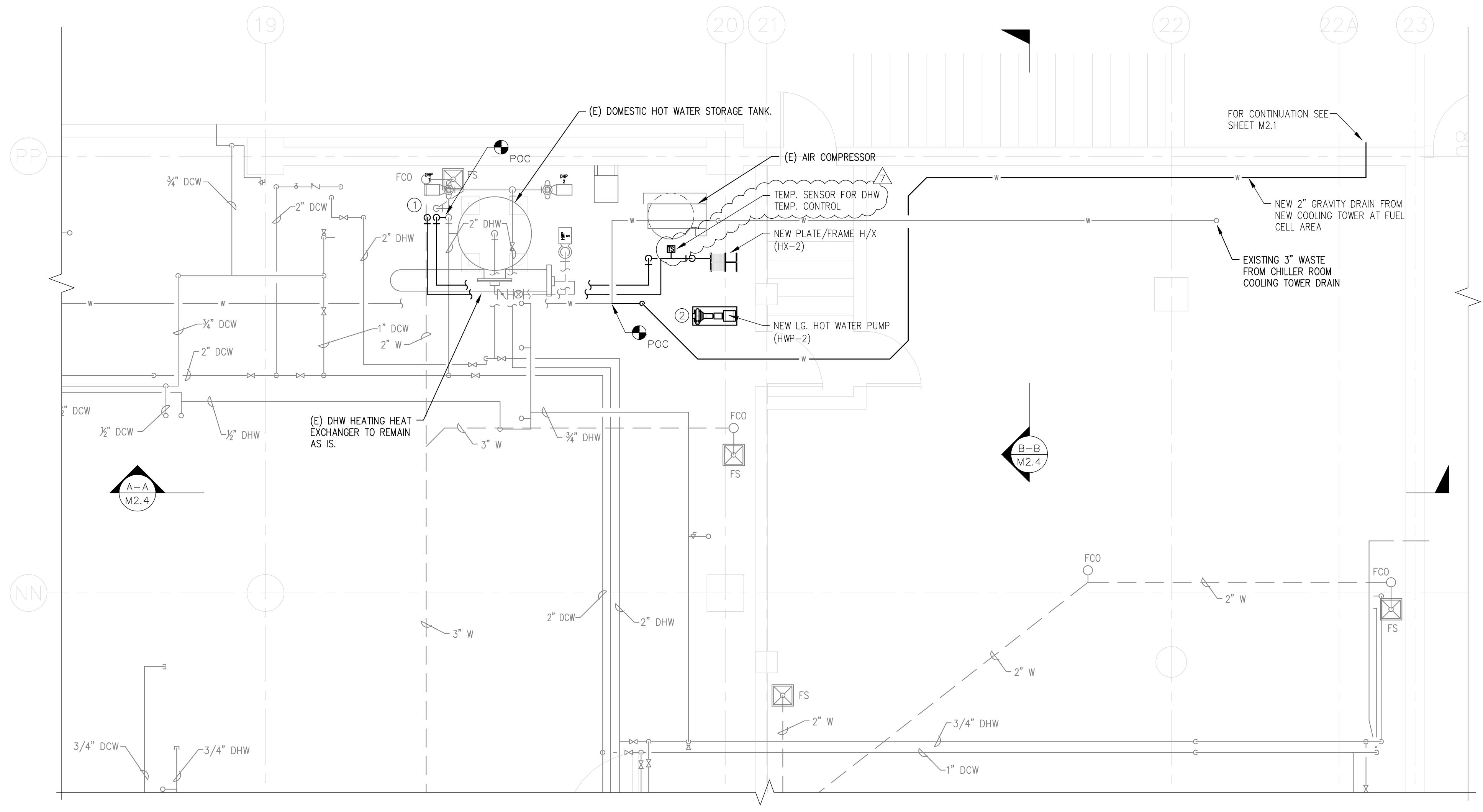
PLUMBING PLAN - SERVICE BUILDING B BOILER ROOM SCALE: 1/4" = 1' - 0"
